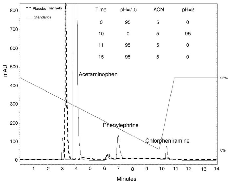
Fig. 1. Chromatogram of the active compounds (acetaminophen, phenylephrine and chlorpheniramine) and excipients sachets at 215 nm with phosphate buffer 10 mM/acetonitrile 95:5 (v/v) in a pH gradient from 7.5 to 2.0 in 10 min on a Discovery CN column (5 μm particle size, 4.6 mm × 250 mm) kept at 35 °C. Detection at 215 nm.
